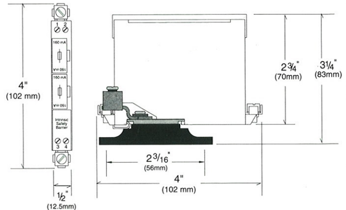
A1-0006 Universal Busbar
