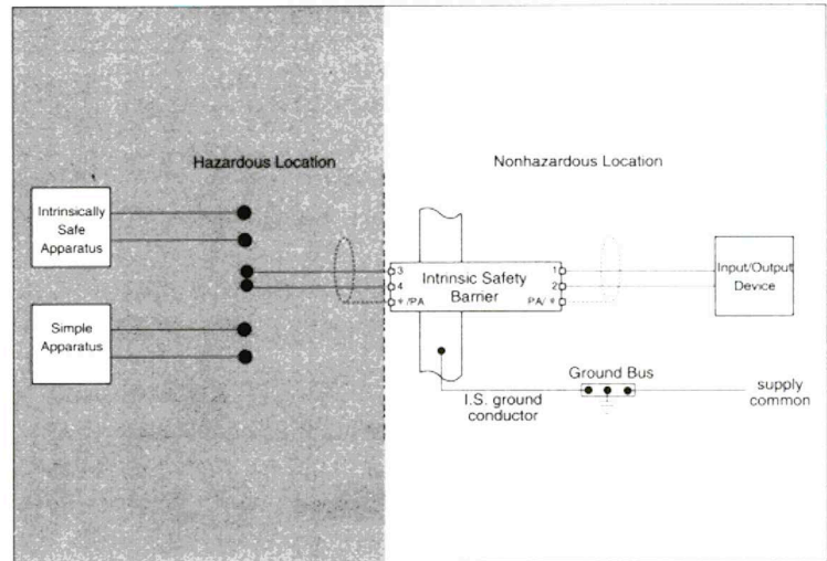
Figure 1. Application of Series 9000 Intrinspak® Intrinsic Safety Barriers
